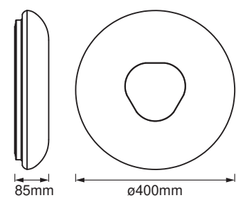
SMART WIFI ORBIS DONUT RD 400 TW WT
