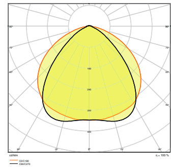
TRUSYS PFM 35W 4000K W DALI
