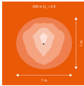
Floodlight Performance 150W SYM R30 simplified isolux diagram
